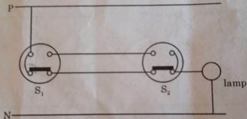
Fig. 2.60 : Schematic diagram
