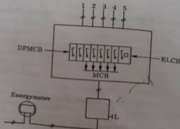
Fig. 2.30: Single line diagram
