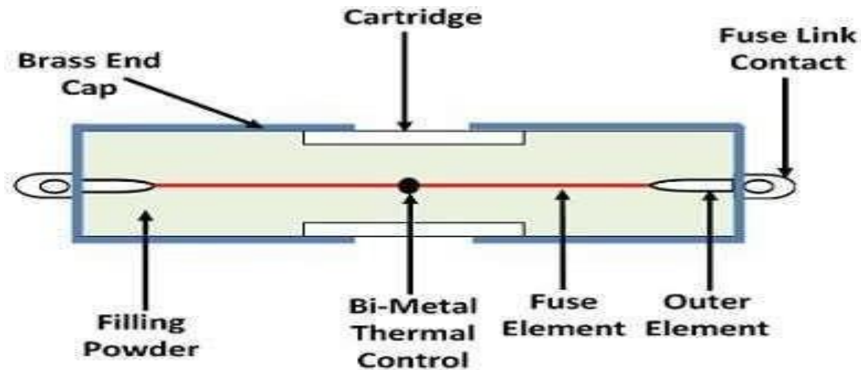
HRC Cartridge Fuse
