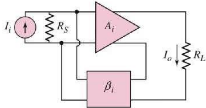
(b) Shunt-series
