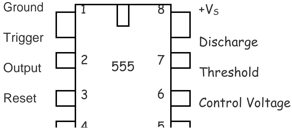
Pin diagram for the 555 timer IC
