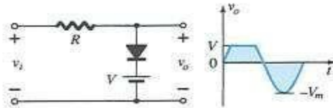
Biased Parallel Clippers (Ideal Diodes)
