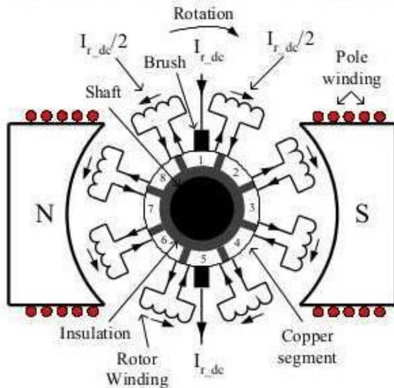
Figure 8.2 Commutator with the rotor coils connections.
