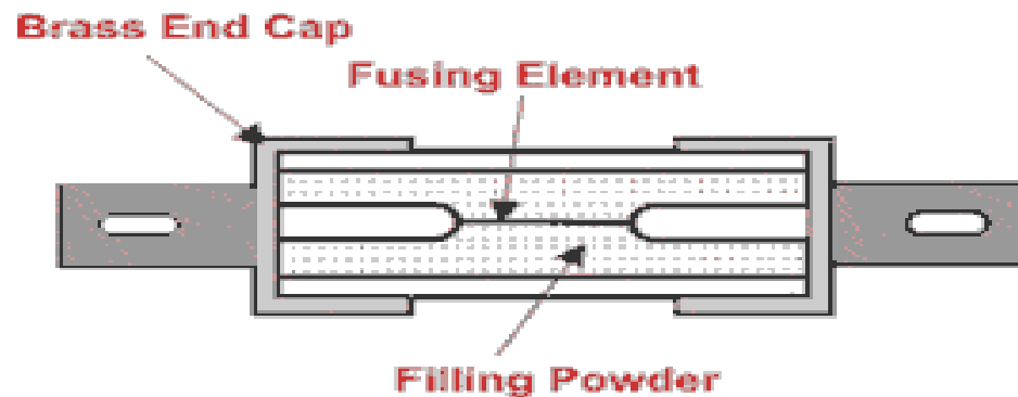
Construction of HRC Fuse
