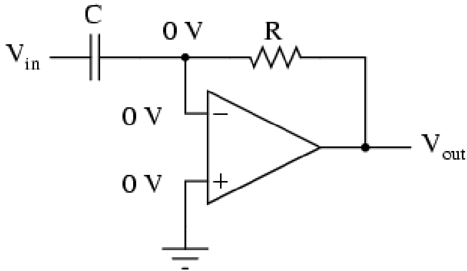
Differentiator
