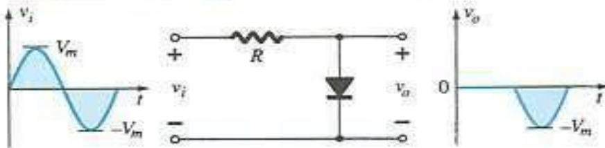
Simple Parallel Clippers (Ideal Diodes)
