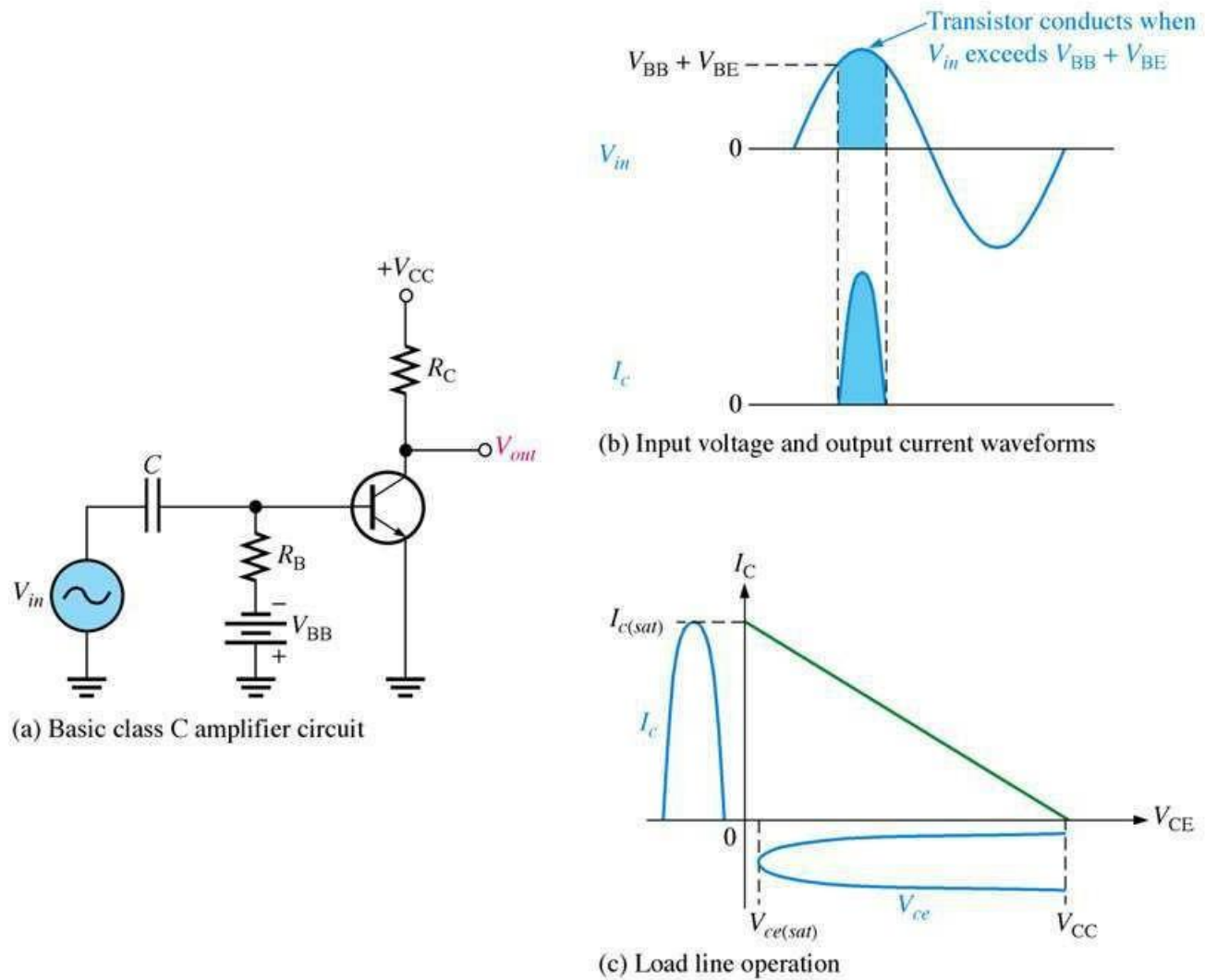
FIGURE 9-23 Basic class C operation.
