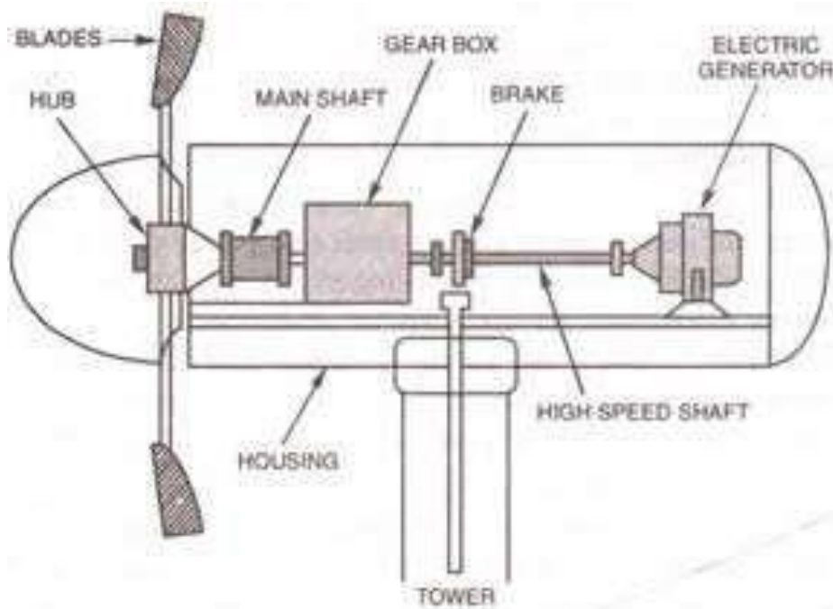
Fig. 7.39. Wind Turbine
