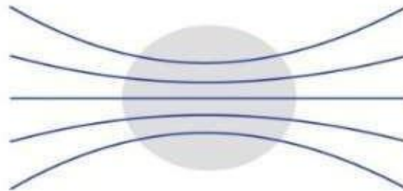
Ferromagnetism
