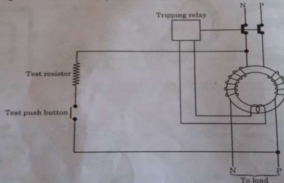
Fig. 3.10 : Circuit of ELCB
