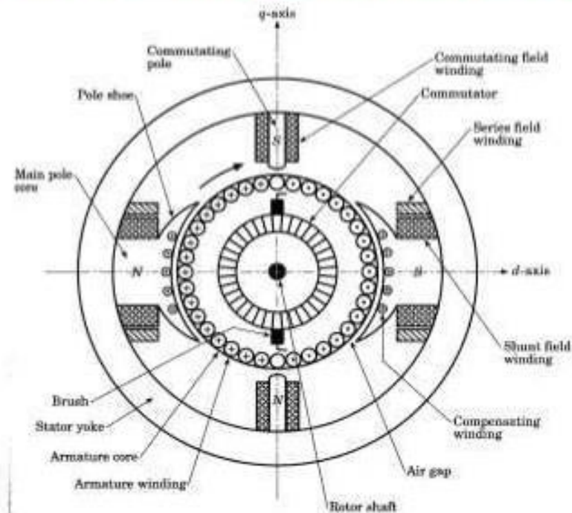
Figure 8.1 General arrangement of a dc machine
