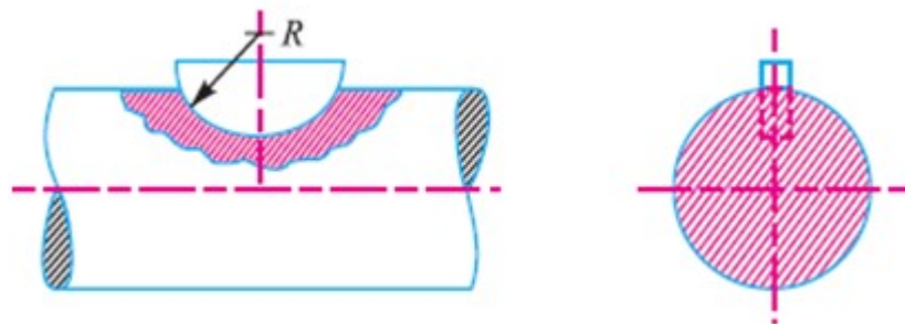
Woodruff Key
