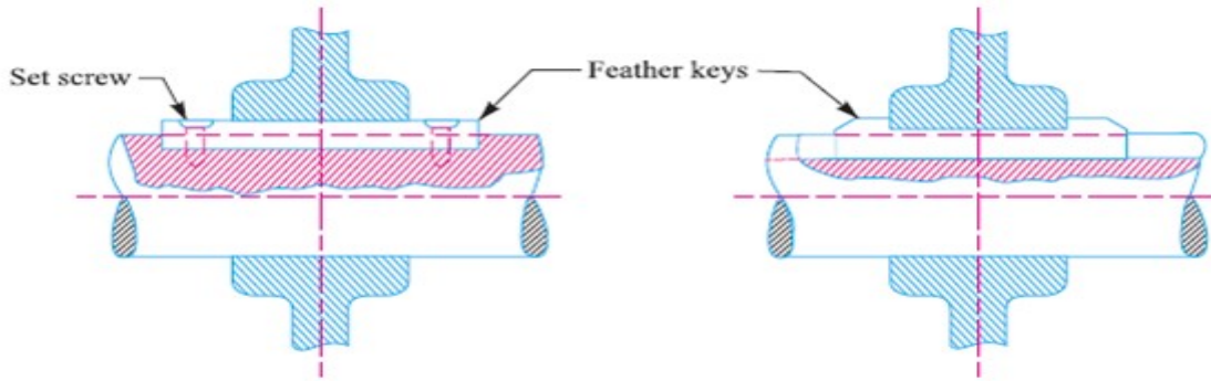
Feather Key
