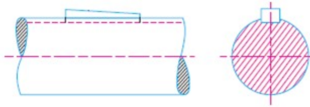
Rectangular Sunk Key
