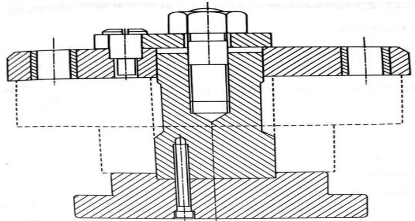
Front View-Full in Section
