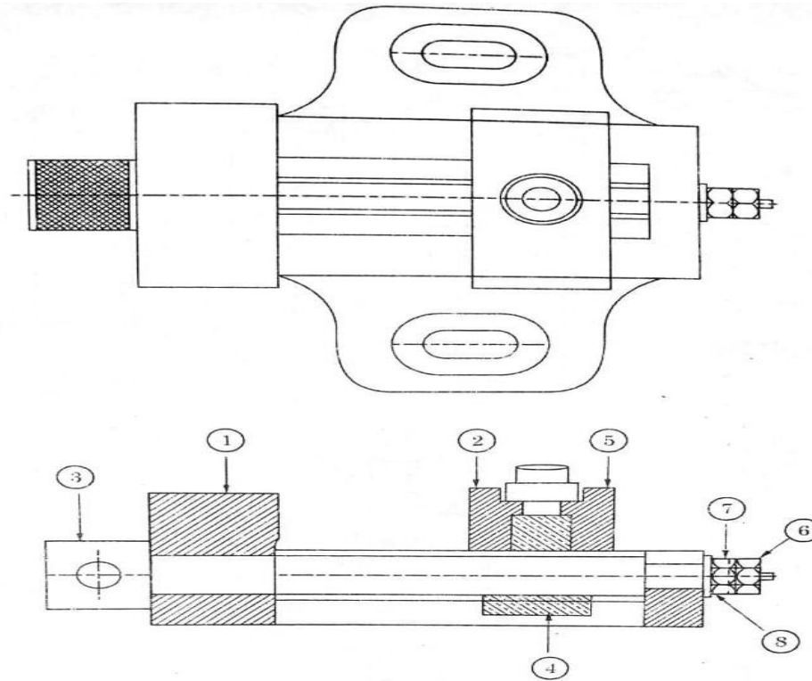
Bill of Materials Machine Vice - Fig. 9.3
